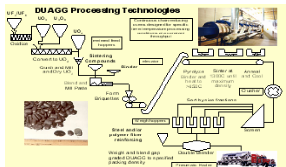
Fig. 2 Ceramics production using the STARMET technology
